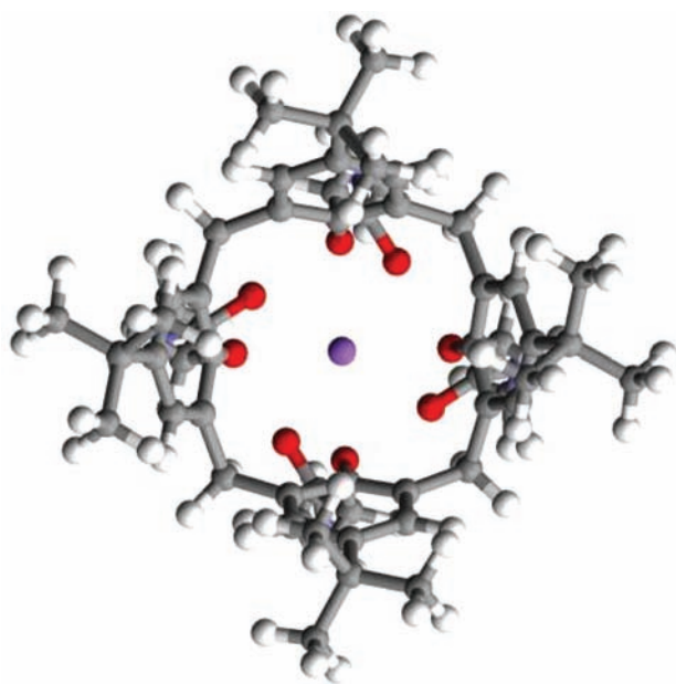
Figure 14. Molecular structure of the \text{Na}^+ complex with L' optimized at the B3LYP/6-311++G(d,p) level of theory.
