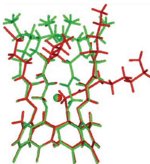
Figure 6. Overlap of the [NaL] + ions from the crystal structures of [NaL]ClO 4 (green) and [NaLMeCN]barb (red). tert -Butyl groups have been omitted for clarity.
