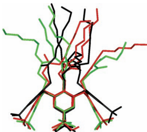
Figure 5. Overlap of the molecules of L from the crystal structures of L ·2MeOH, (black), the MeCN adduct LMeCN (red), and the sodium complex [NaL]ClO 4 (green). Hydrogen atoms have been omitted for clarity.
