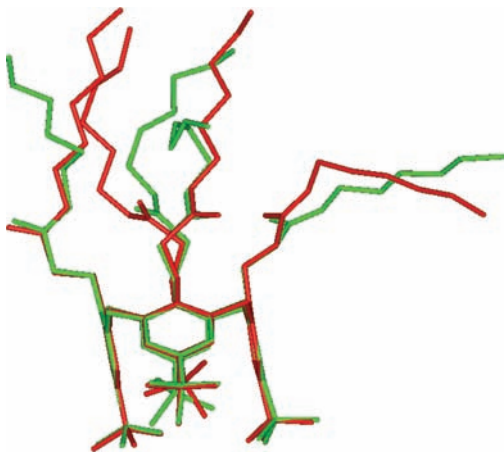
Figure 2. Overlap of the molecules of L from the crystal structures of the solvent-free crystal (green) and the MeOH solvate (red), showing almost identical cone geometry in the two crystals. Hydrogen atoms as well as minor components of all disordered groups have been omitted for clarity.
