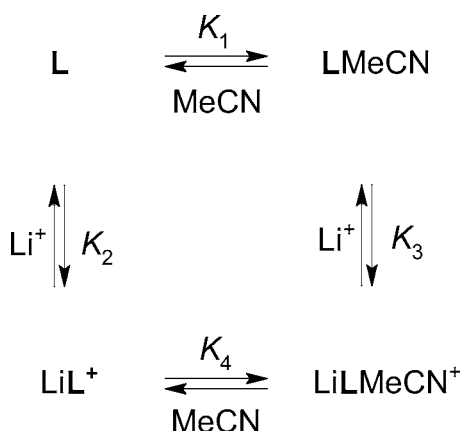
Scheme 2. Chemical Equilibria Corresponding to the Binding of \text{Li}^+ Cation by L
