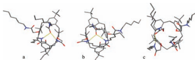
Figure 3. Intramolecular hydrogen bonding in crystal structures of (a) a solvent-free crystal of L, (b) the MeOH solvate L·2MeOH, and (c) the LMeCN adduct. Hydrogen atoms bonded to carbon atoms of L and solvent molecules have been omitted for clarity.
